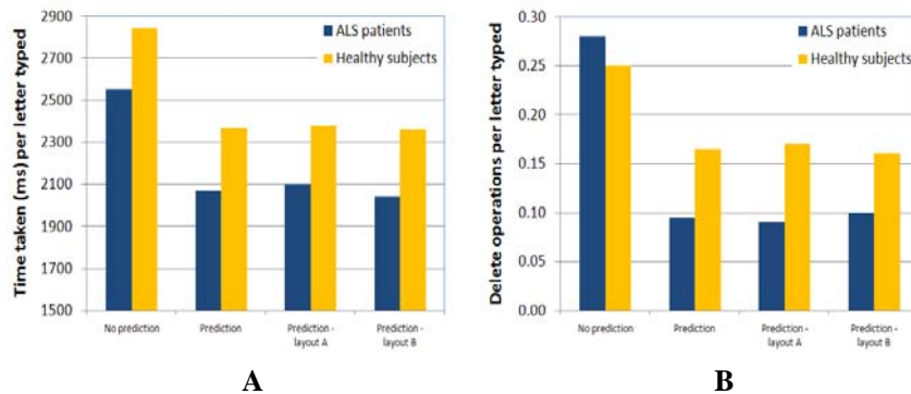
Figure 2: (A) Time taken and (B) delete operations per letter typed for the ALS patients and the non-disabled subjects. Each chart compares the “no word prediction” and “word prediction” (1, 2, or 3 words) conditions (two leftmost groups of columns). Among the “word prediction” trials, layouts A and B are compared (two rightmost groups of columns).
