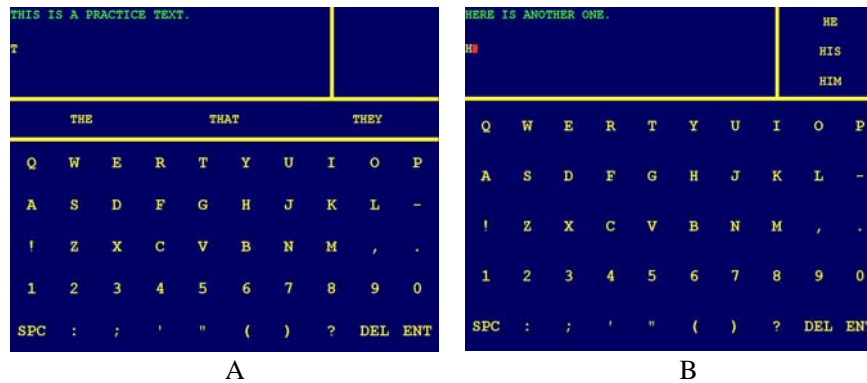
Figure 1: The two interface layouts used in the preliminary study. The subjects' task was to type the text shown at the top of the screen. (A) Word suggestions shown below the text field; (B) word predictions shown to the right of the text field.
