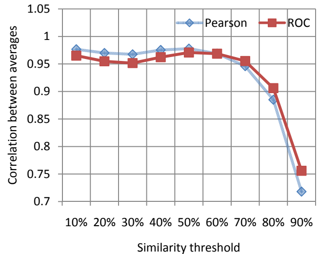
Figure 9. Correlation coefficient between average informativeness and average guidance across the eight dimensions, shown as a function of the similarity threshold. For threshold up to 70%, there exists a strong positive correlation ( r > 0.95 ).
