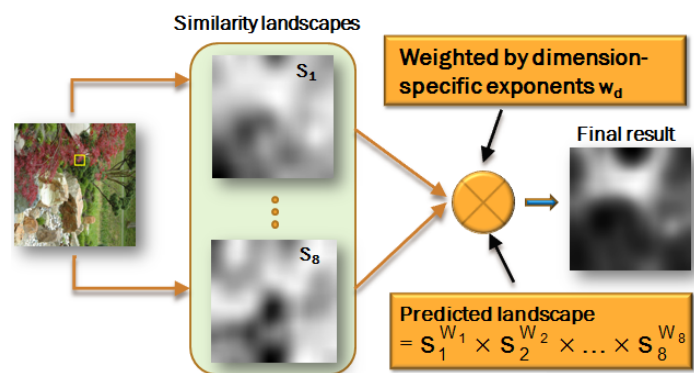
Figure 11. Schematic of model operation. From the similarity landscapes, weighting across dimensions is computed based on informativeness. Afterwards, similarity landscapes are integrated using the weighted product method.
