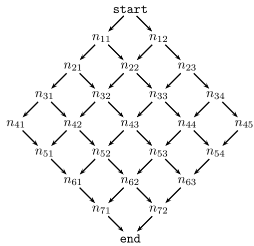
Figure 1: A serious DAG.
