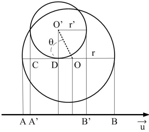
Fig. 2. Projections of two spheres onto a random unit vector
