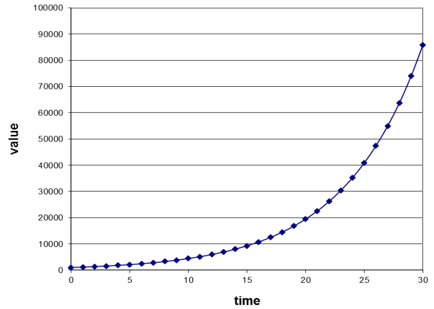
Exponential Growth
