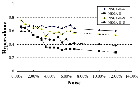
Fig. 10. Hypervolume (lin318, Normal Distribution Noise)
