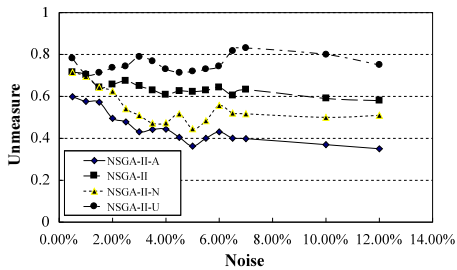
Fig. 22. U-metric (lin318, Normal Dist. Noise)
