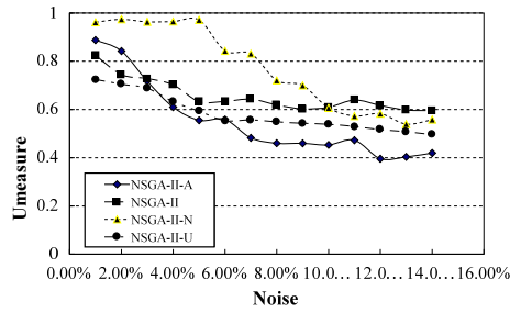
Fig. 21. U-metric (pr226, Uniform Dist. Noise)
