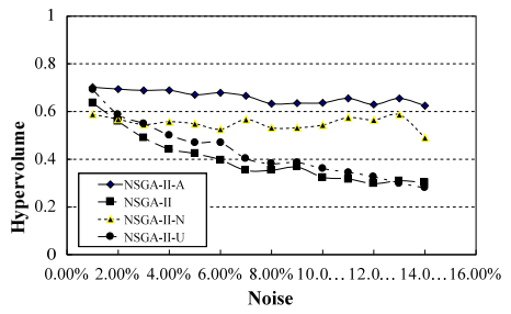
Fig. 9. Hypervolume (pr226, Uniform Distribution Noise)
