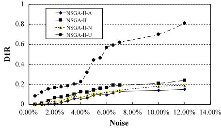
Fig. 16. D1_R (lin318, Normal Dist. Noise)
