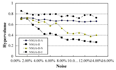
Fig. 7. Hypervolume (ch130, Uniform Distribution Noise)
