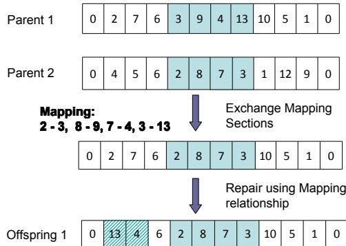
Fig. 2. An Example Crossover (PMX) Process
