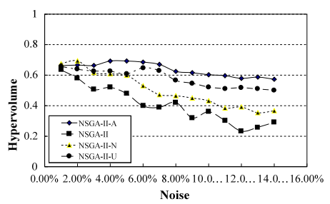
Fig. 11. Hypervolume (lin318, Uniform Distribution Noise)
