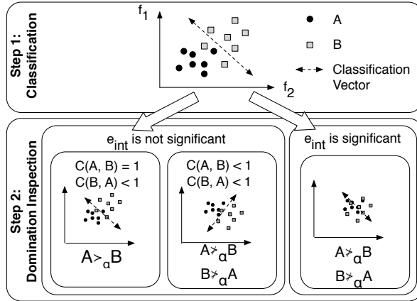
Fig. 4. An Example Process to determine the \alpha -Dominance Relationship between two individuals ( A and B )
