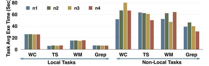
Fig. 4: Task average execution time in Setting 3
