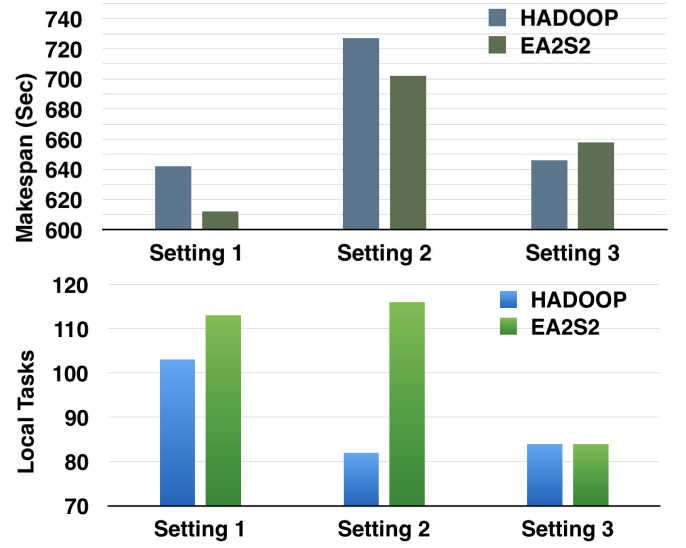
Fig. 7: Makespan and local task amount of 10 nodes cluster
