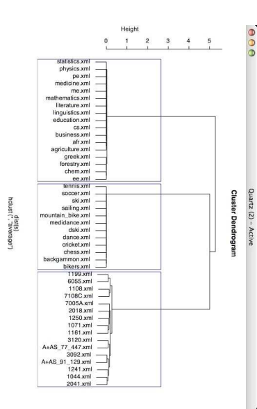
Figure 3: Niagara Data Set Clusters (Strong Distance Measure)
