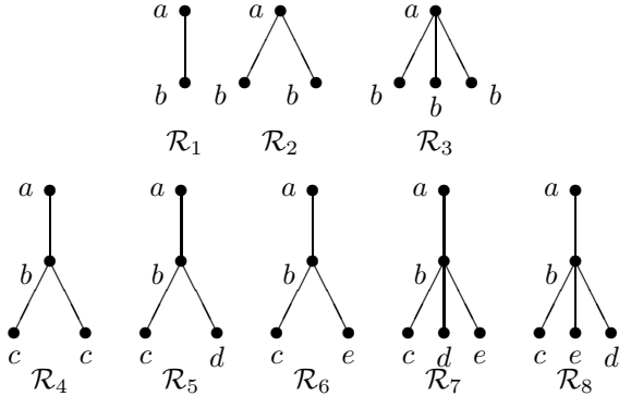
Figure 1: Examples of Labeled Rooted Trees
